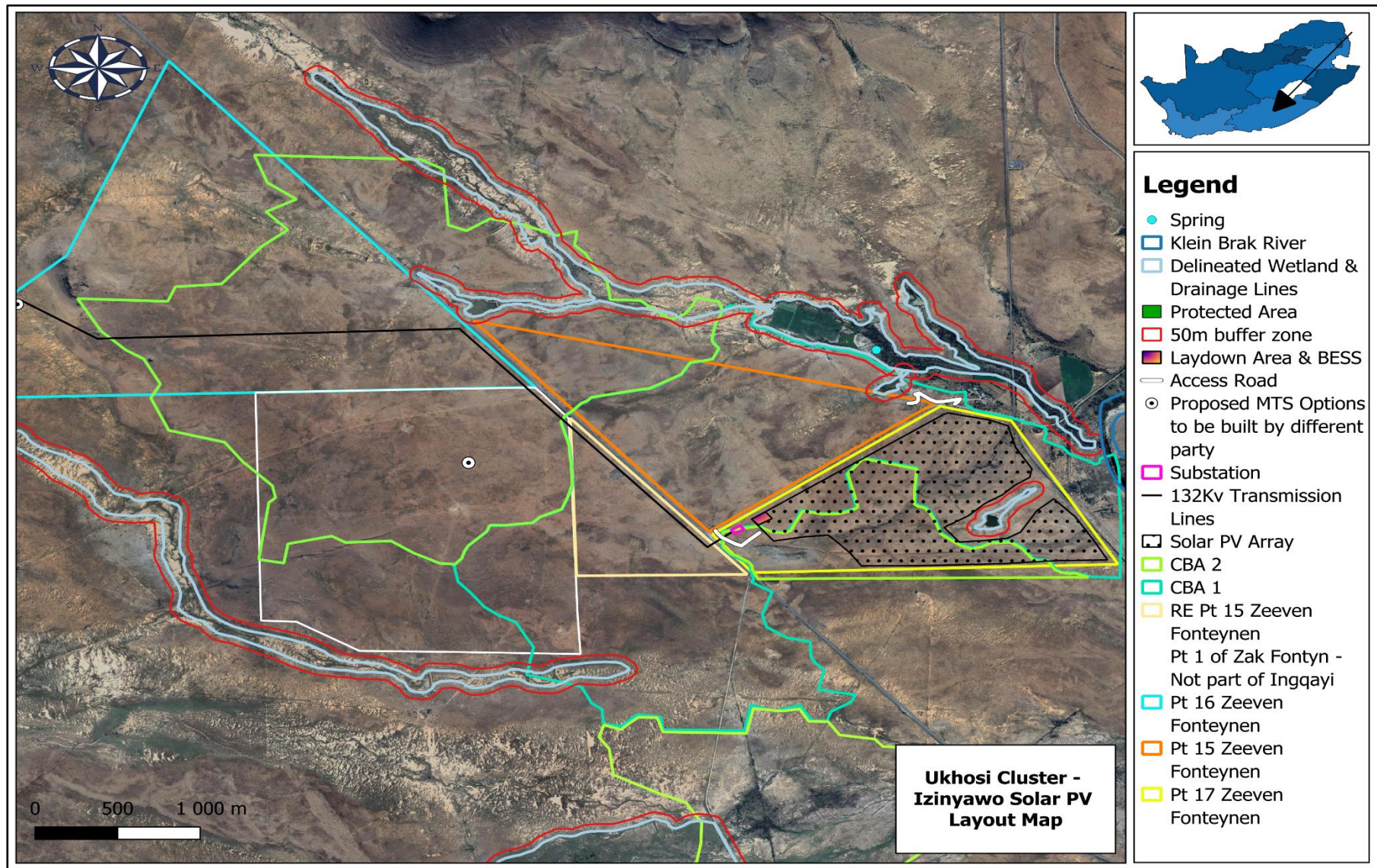
Figure 2: Izinyawo Solar – Layout Map
